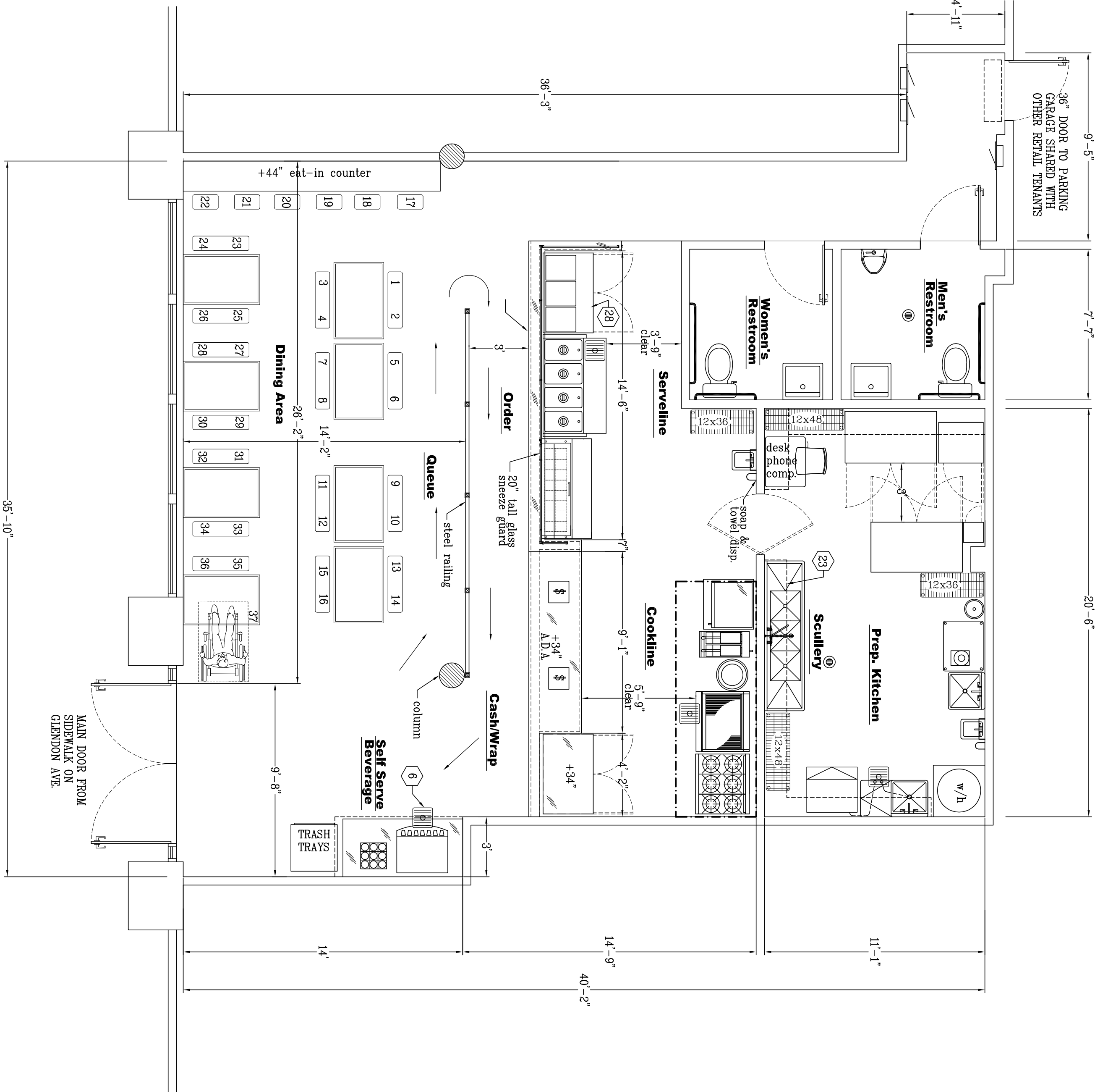
RESTAURANT FLOOR PLAN
